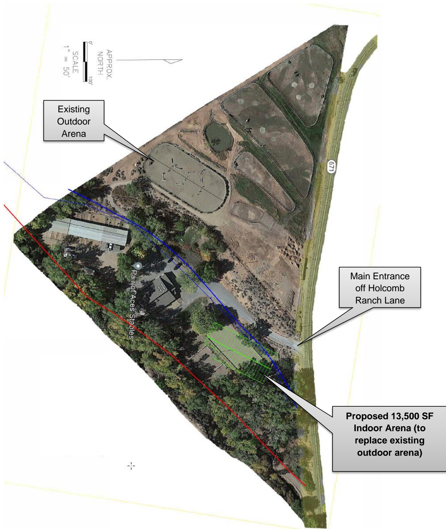
Site Plan
