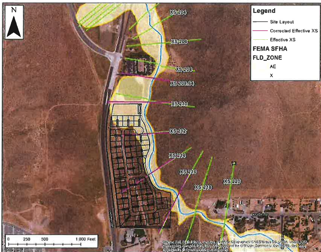
Figure 4. HEC-RAS Model Cross Sections
