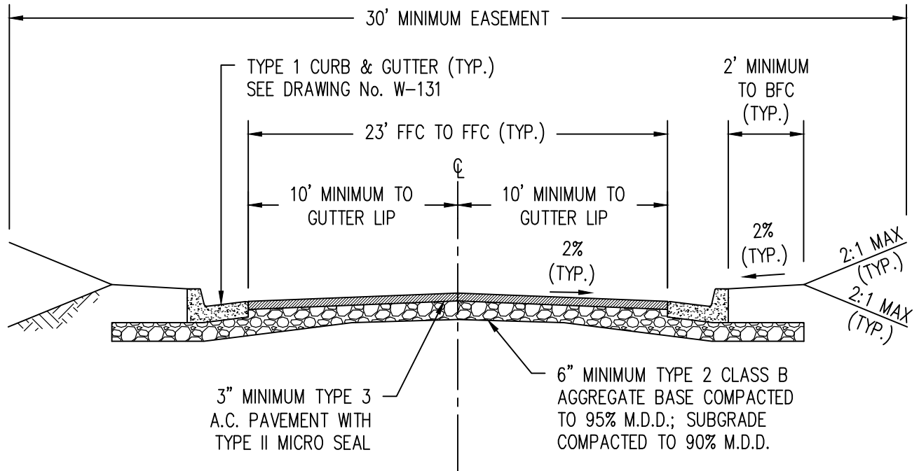
TYPICAL SECTION
